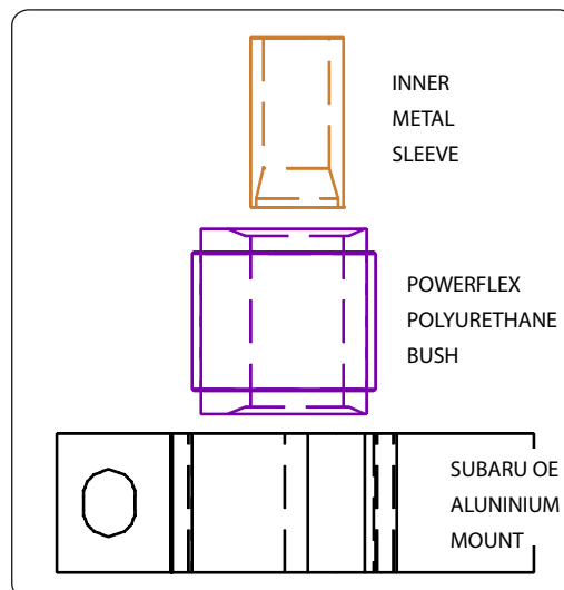
Fig 1. Exploded View
